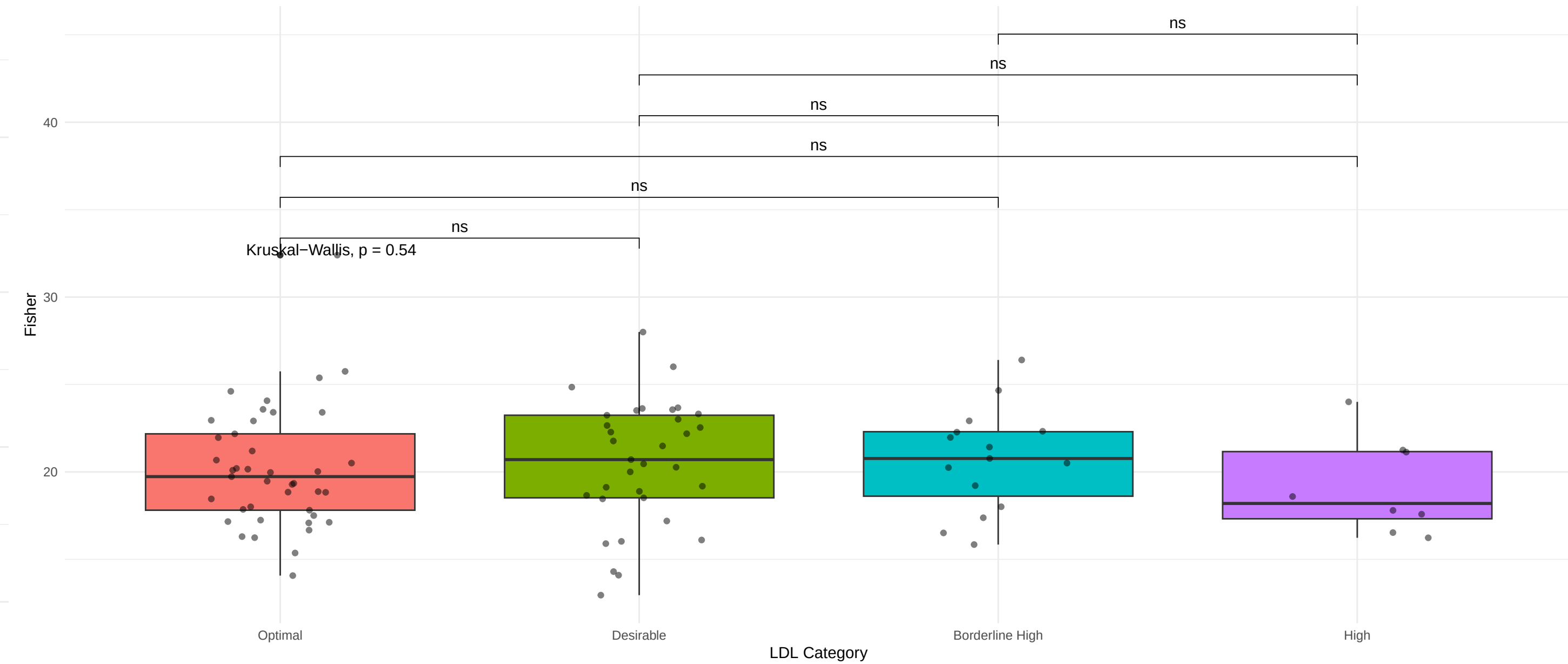
Fisher Diversity by LDL Category
